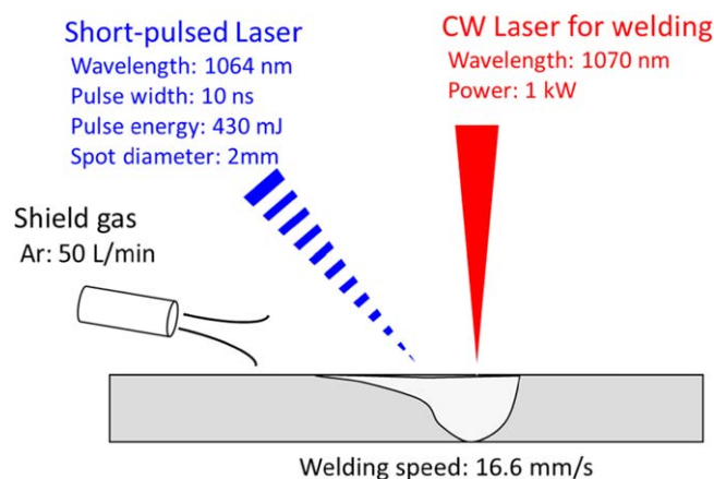
Figure 1. Experimental setup for laser welding.
