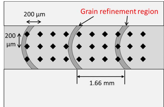
Figure 4. Schematic of measured positions for the hardness test.
